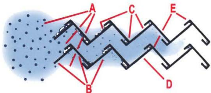
Cross Section View of Peerless Vane Element
